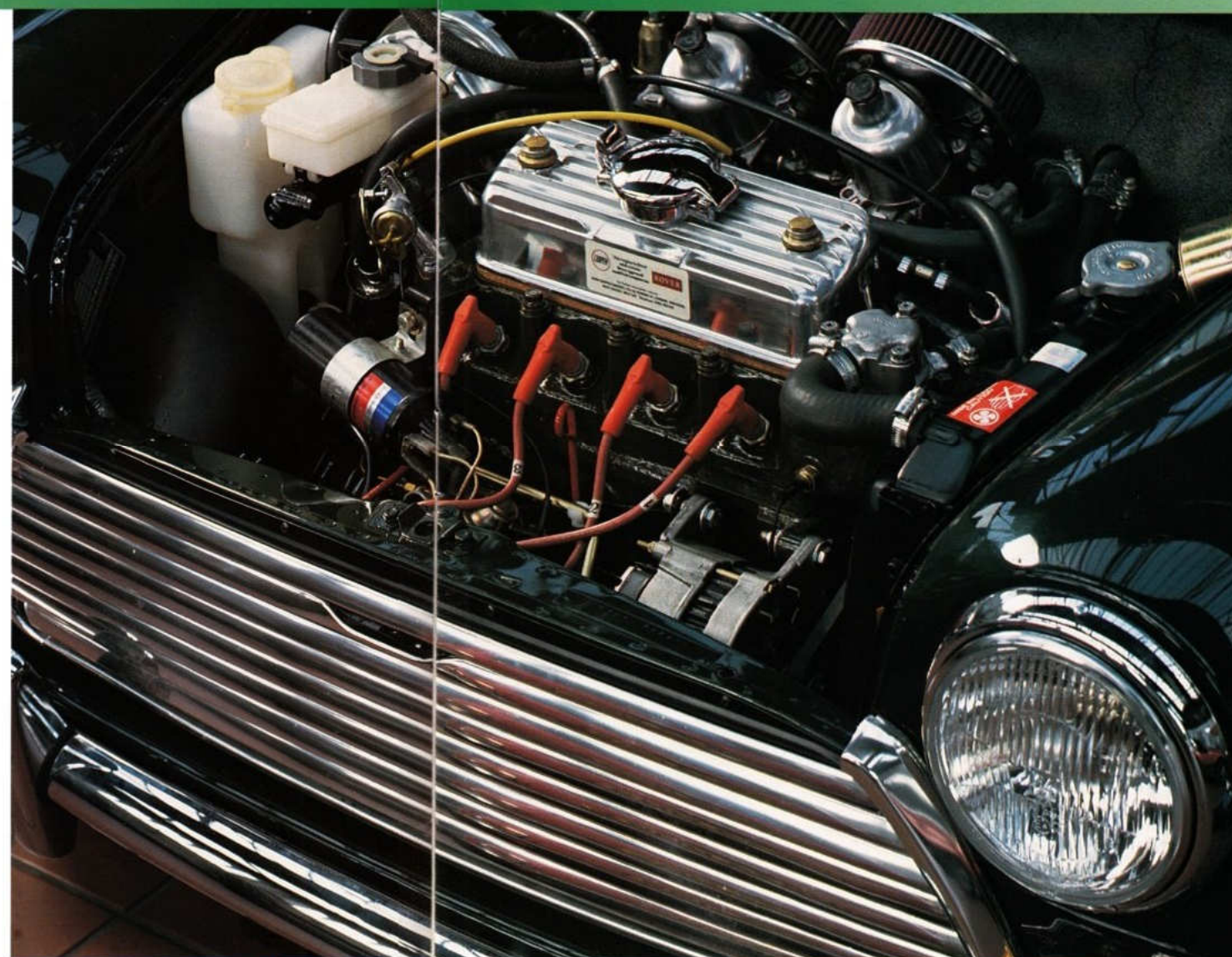
The John Cooper Si Pack (Part No: MCC 1275 ST)
